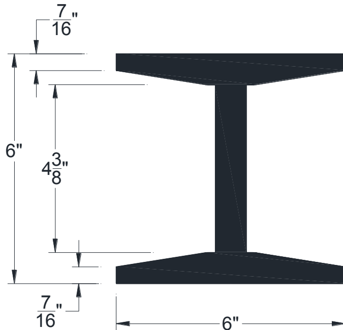
SECTIONAL VIEW
