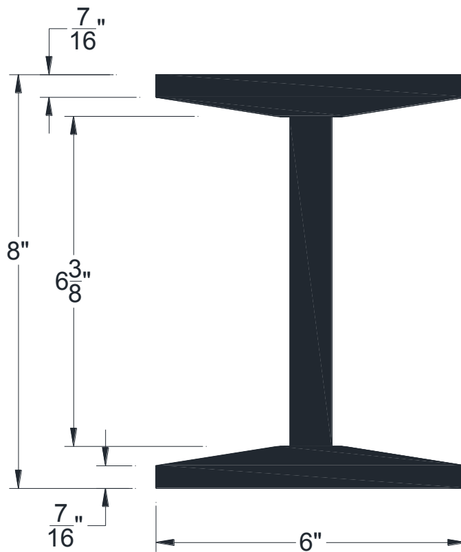
SECTIONAL VIEW
