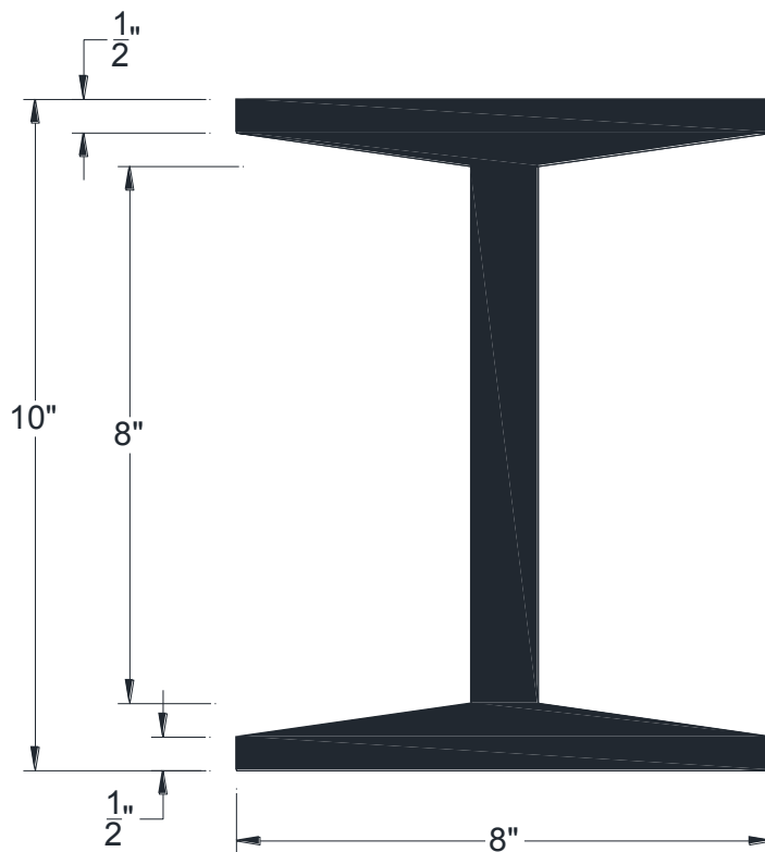
SECTIONAL VIEW
