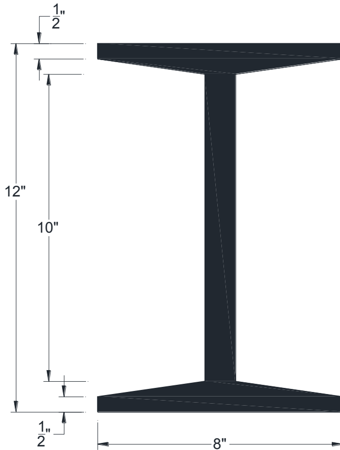
SECTIONAL VIEW
