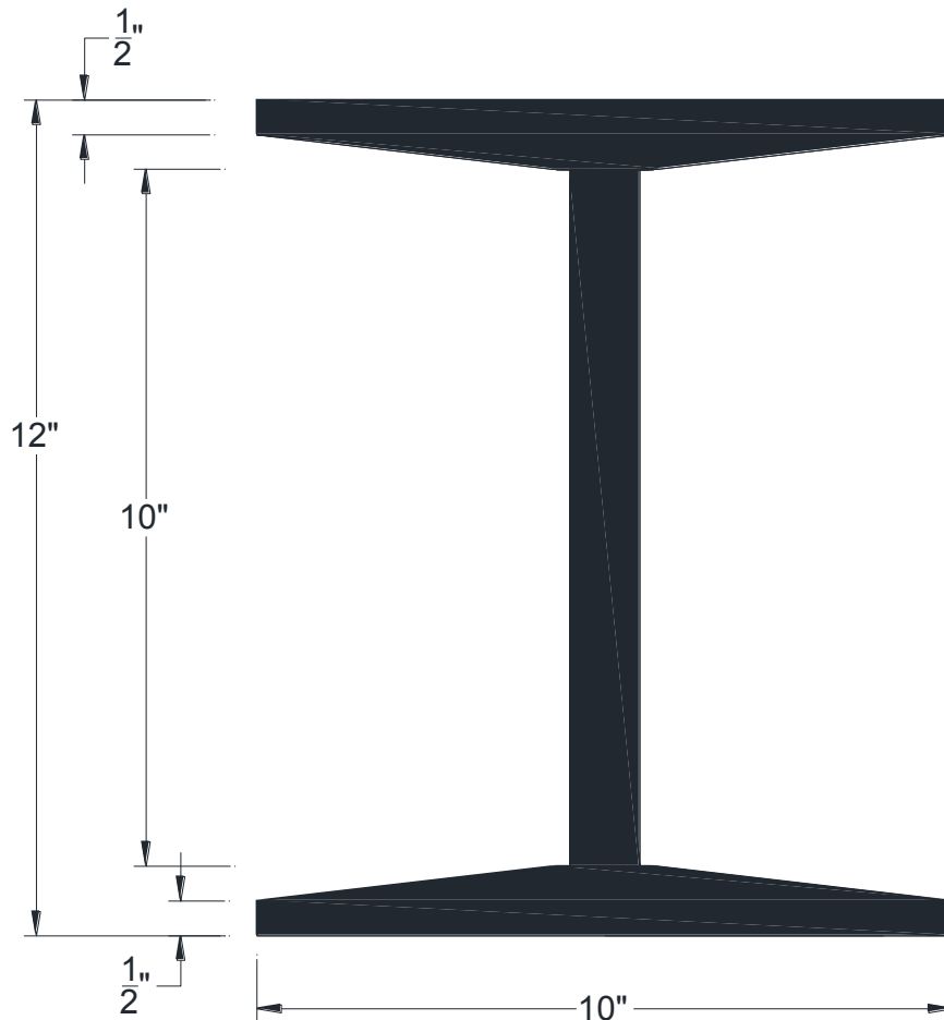
SECTIONAL VIEW
