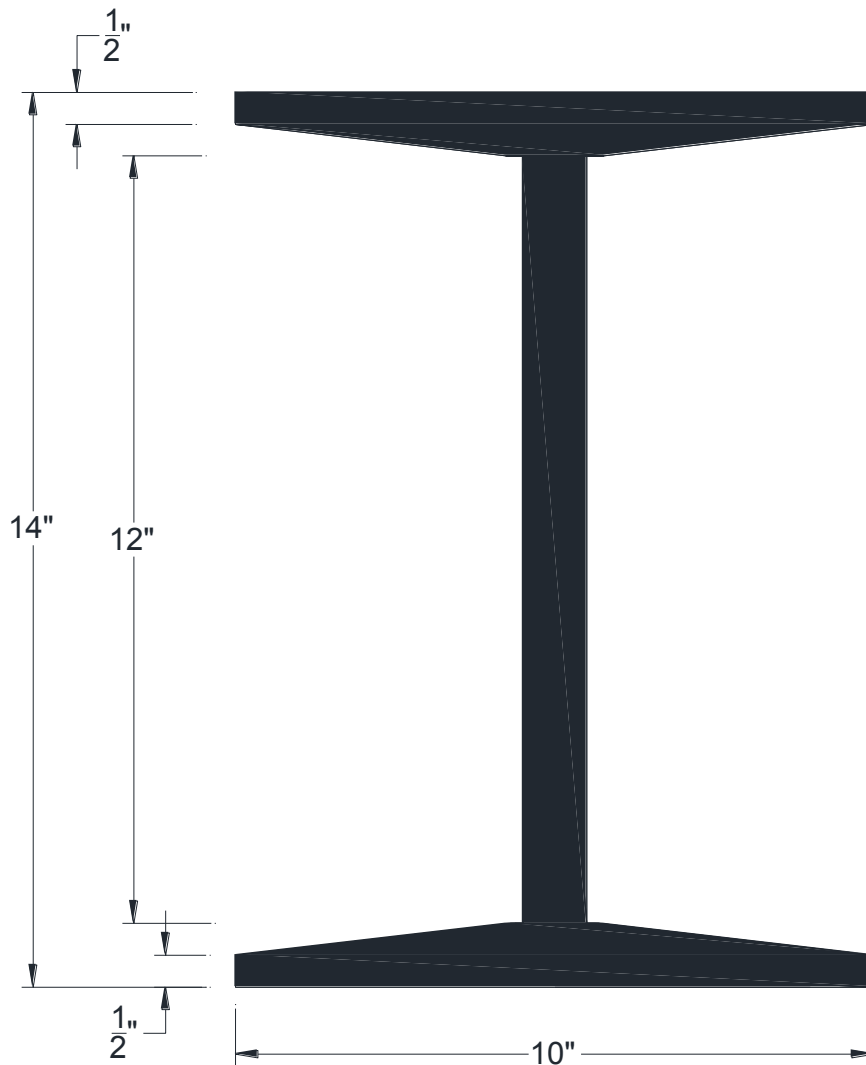
SECTIONAL VIEW
