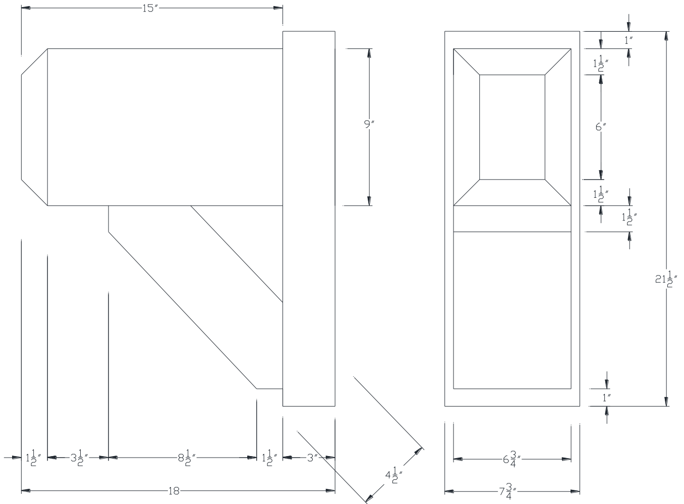
SIDE VIEW
