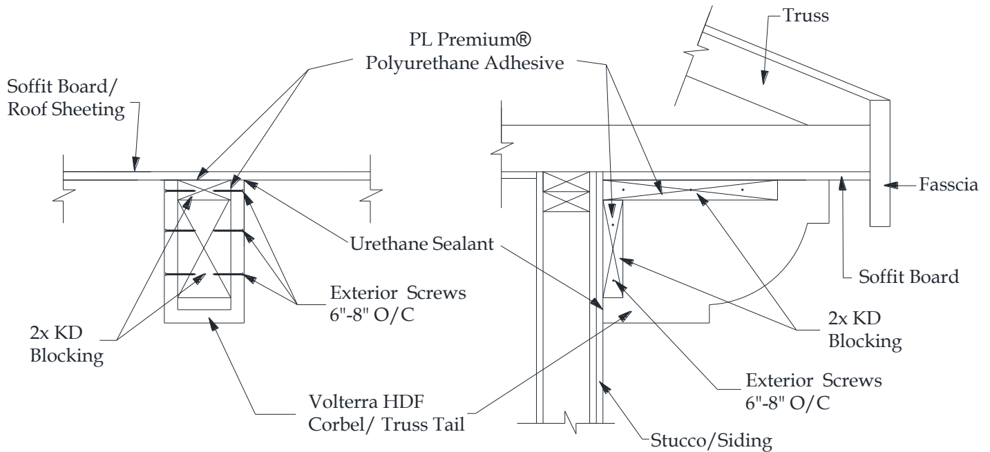
Sectional View
