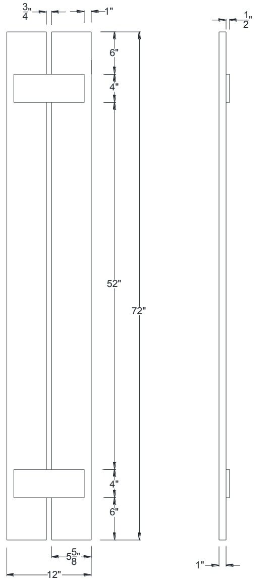
FRONT VIEW
