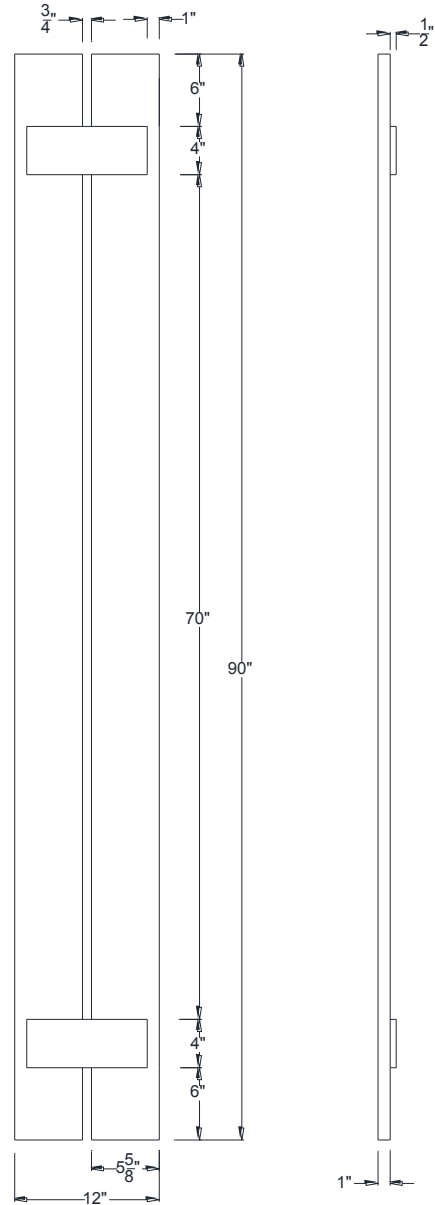
FRONT VIEW
