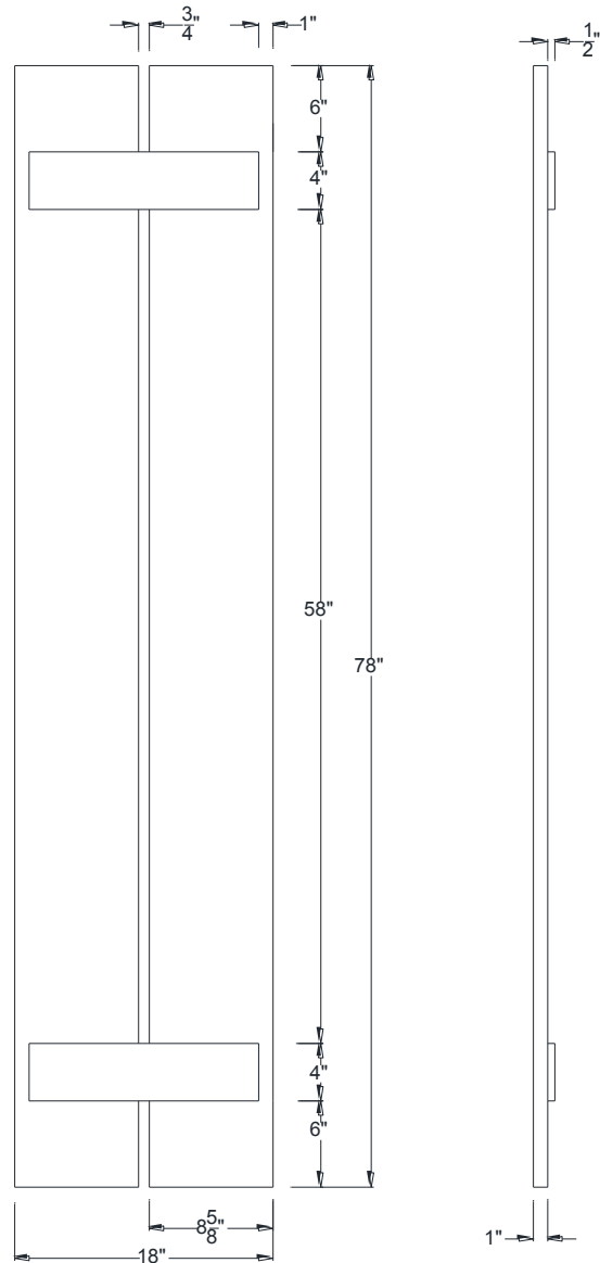
FRONT VIEW
