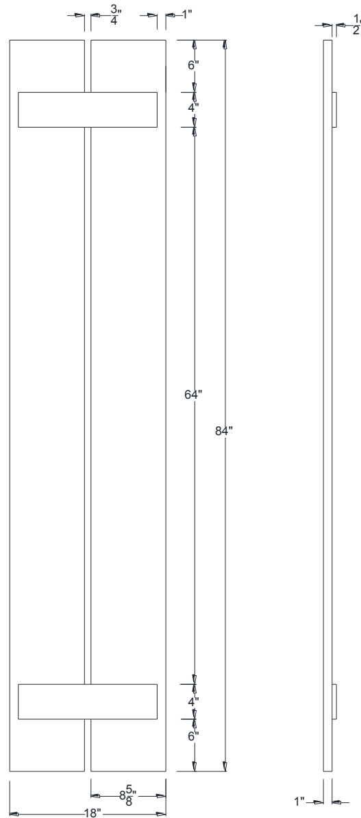
FRONT VIEW
