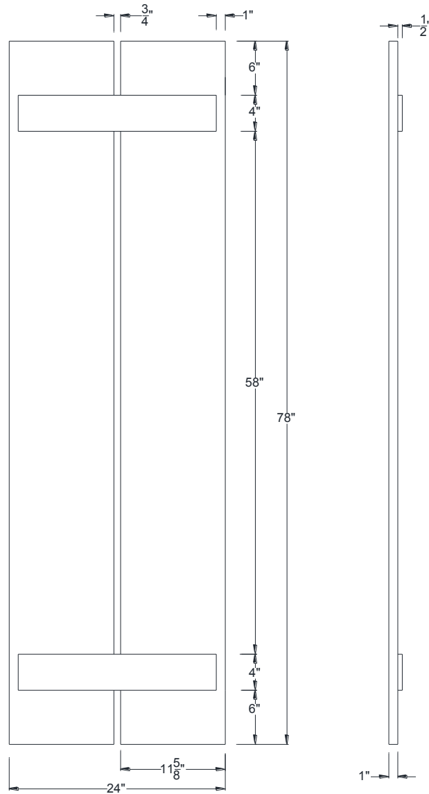
FRONT VIEW
