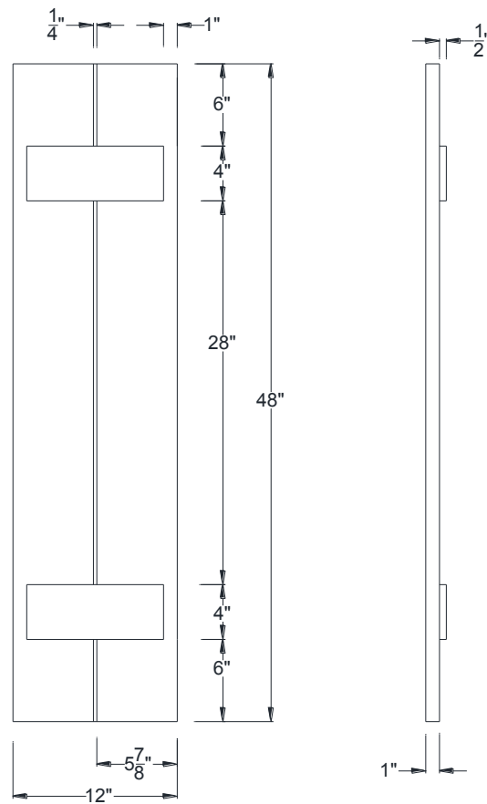
FRONT VIEW
