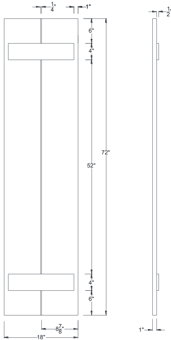
FRONT VIEW
