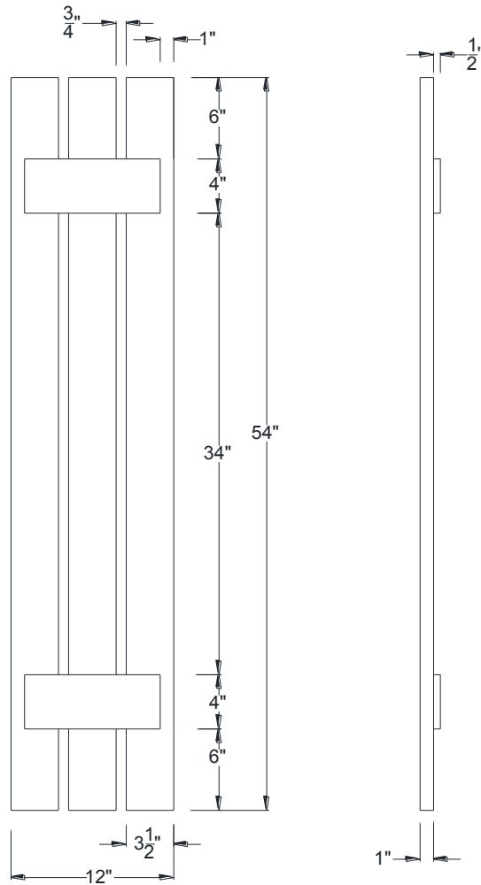
FRONT VIEW
