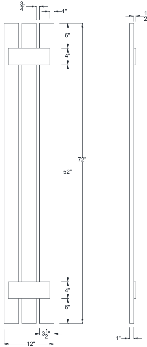
FRONT VIEW
