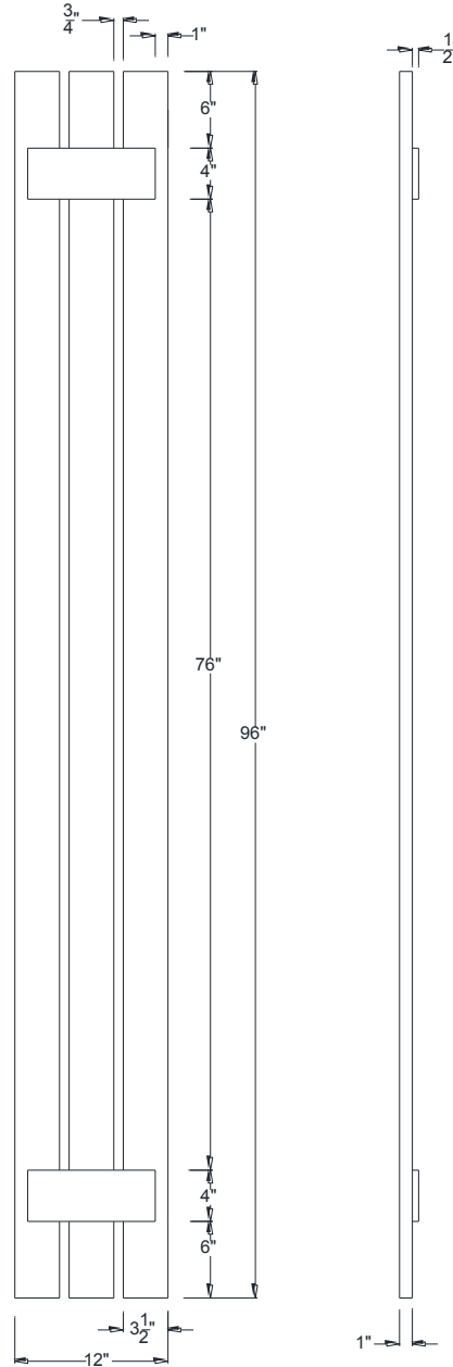
FRONT VIEW
