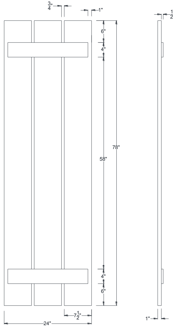
FRONT VIEW
