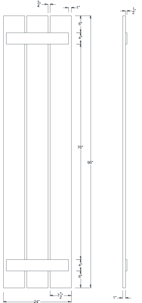
FRONT VIEW
