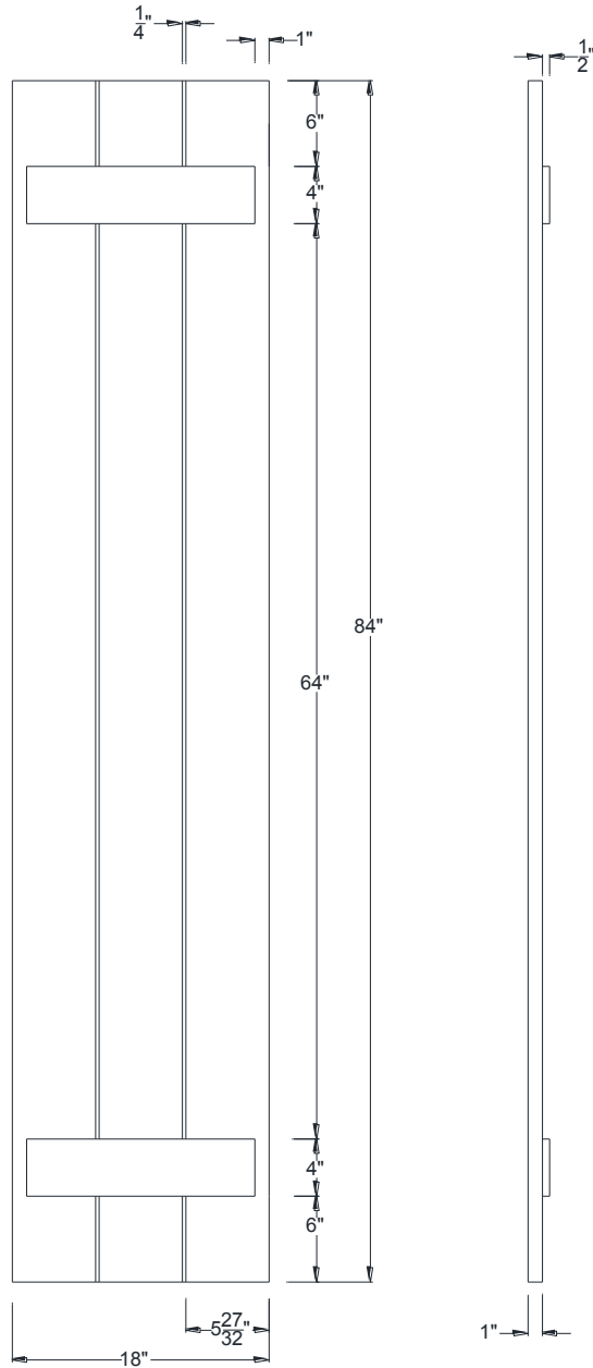
FRONT VIEW
