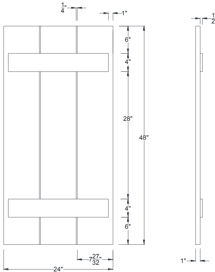
FRONT VIEW
