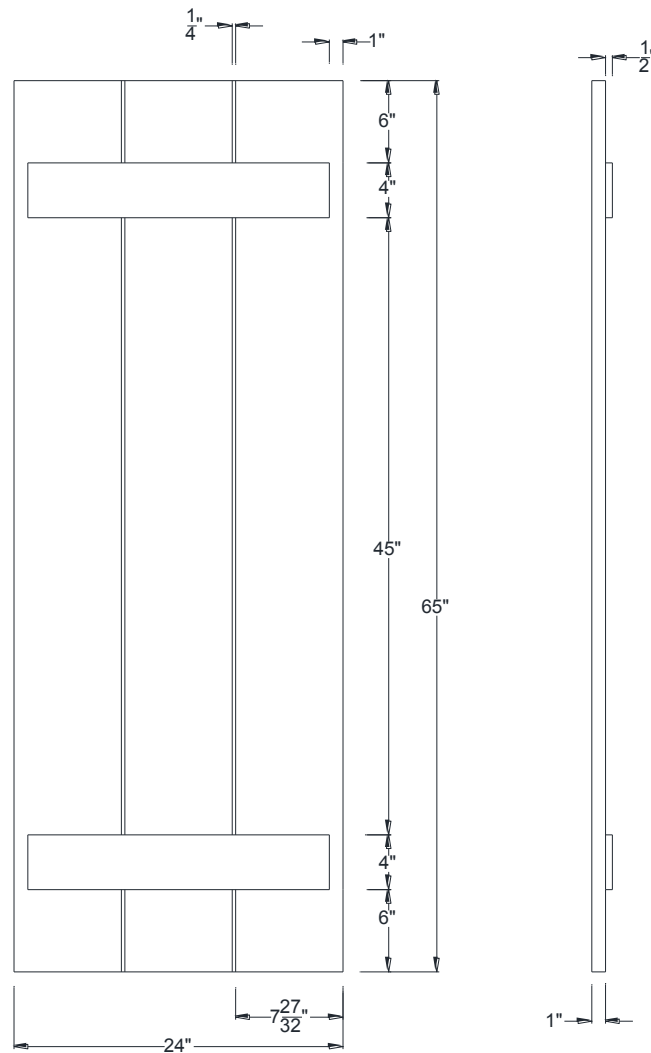
FRONT VIEW
