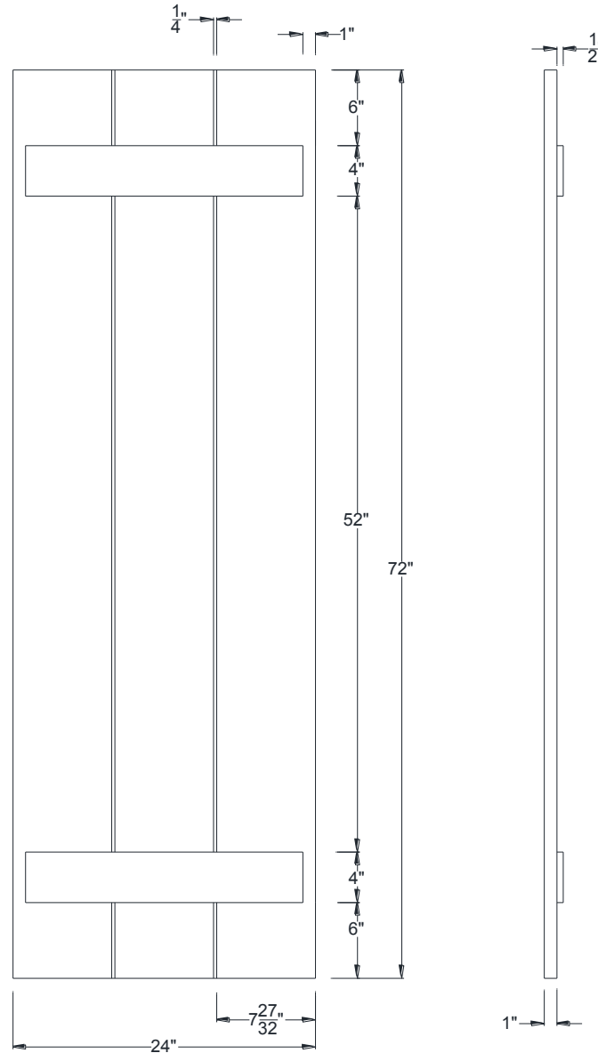
FRONT VIEW
