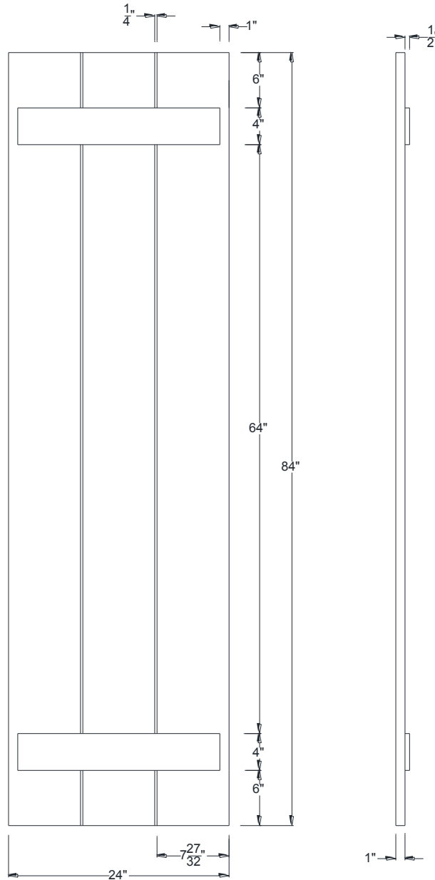
FRONT VIEW
