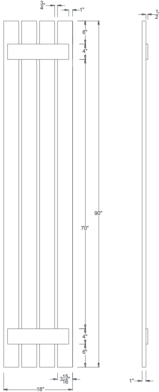
FRONT VIEW
