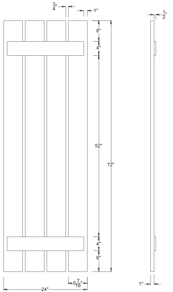
FRONT VIEW
