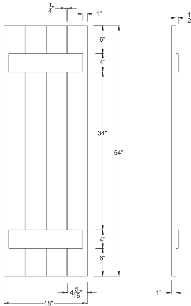
FRONT VIEW
