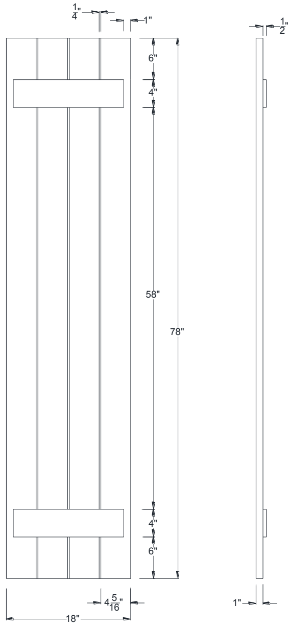
FRONT VIEW
