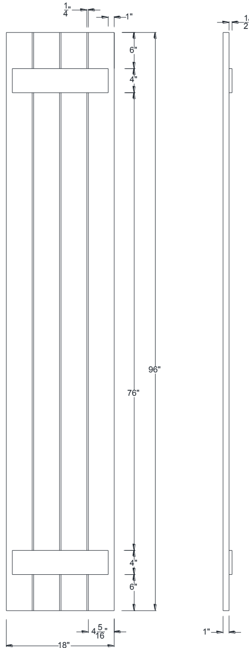
FRONT VIEW
