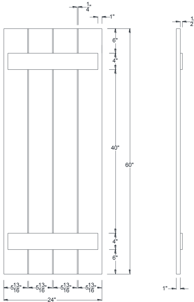
FRONT VIEW
