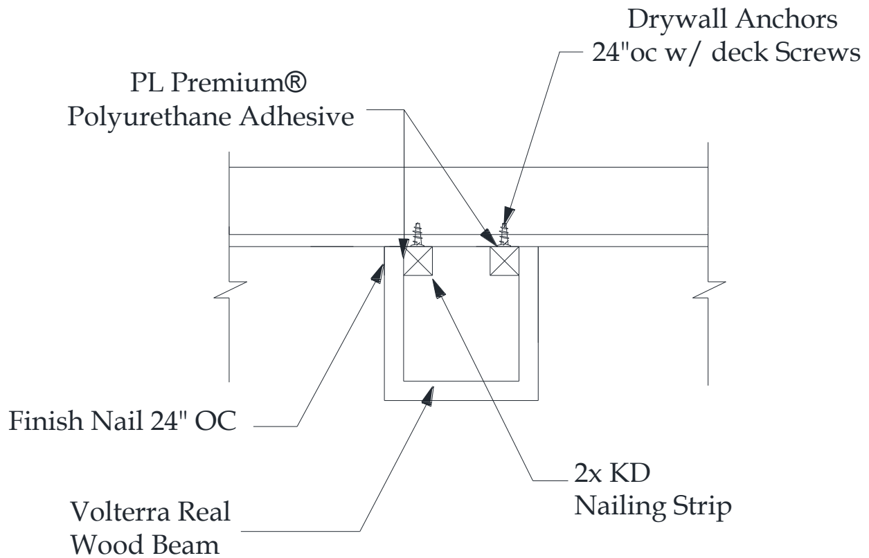
SECTIONAL VIEW
