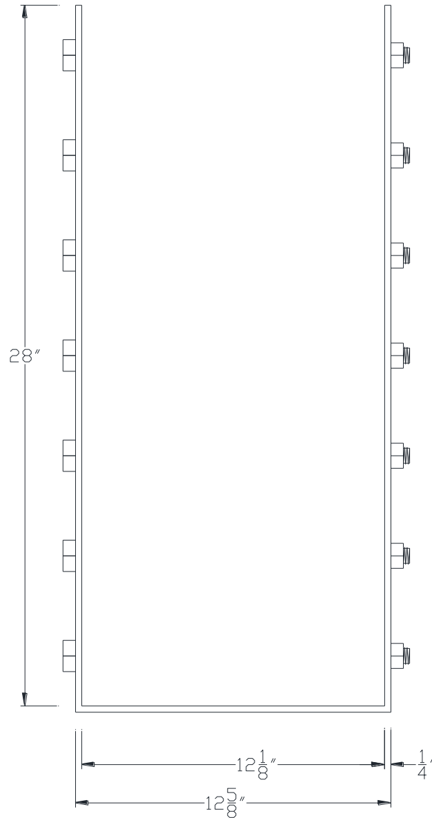
FRONT VIEW
