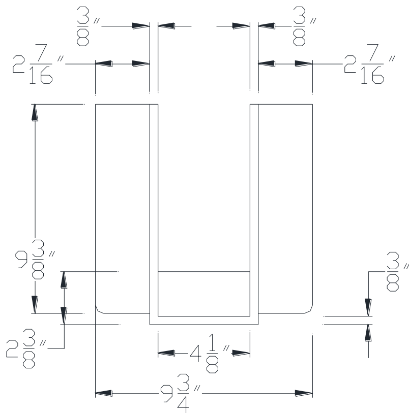
FRONT VIEW
