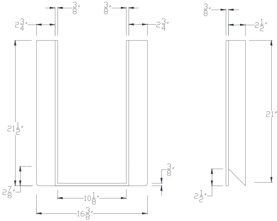
FRONT VIEW
