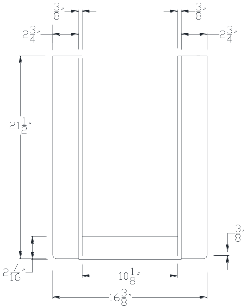
FRONT VIEW
