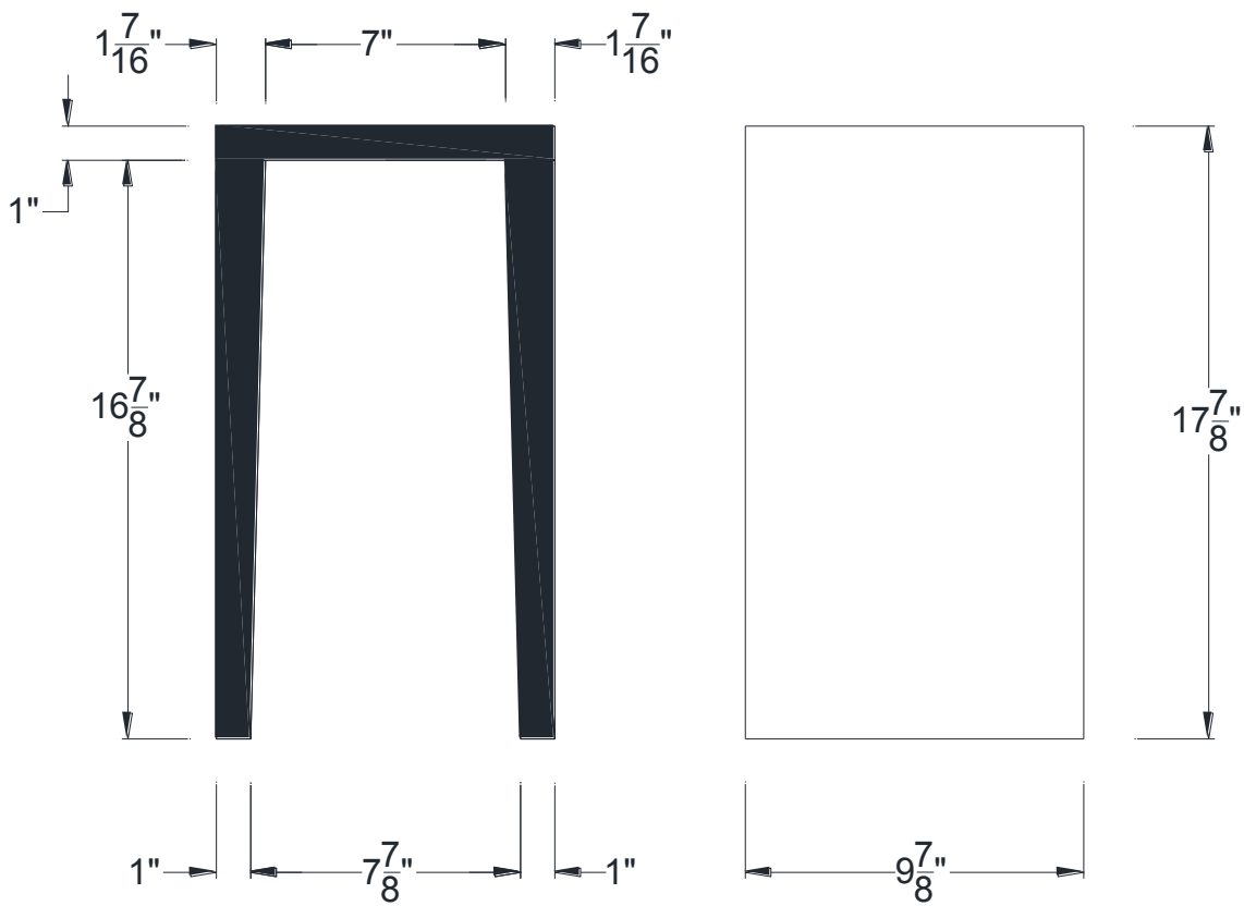
SECTIONAL VIEW
