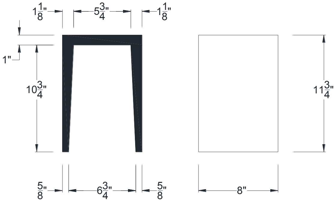
SECTIONAL VIEW
