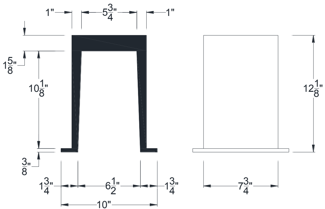
SECTIONAL VIEW
