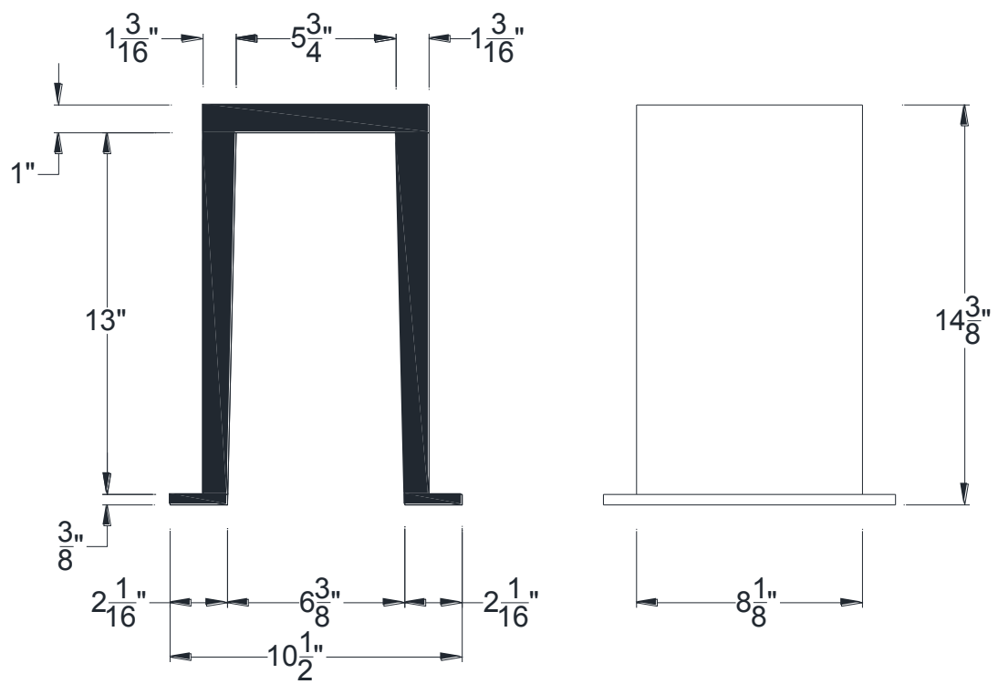
SECTIONAL VIEW
