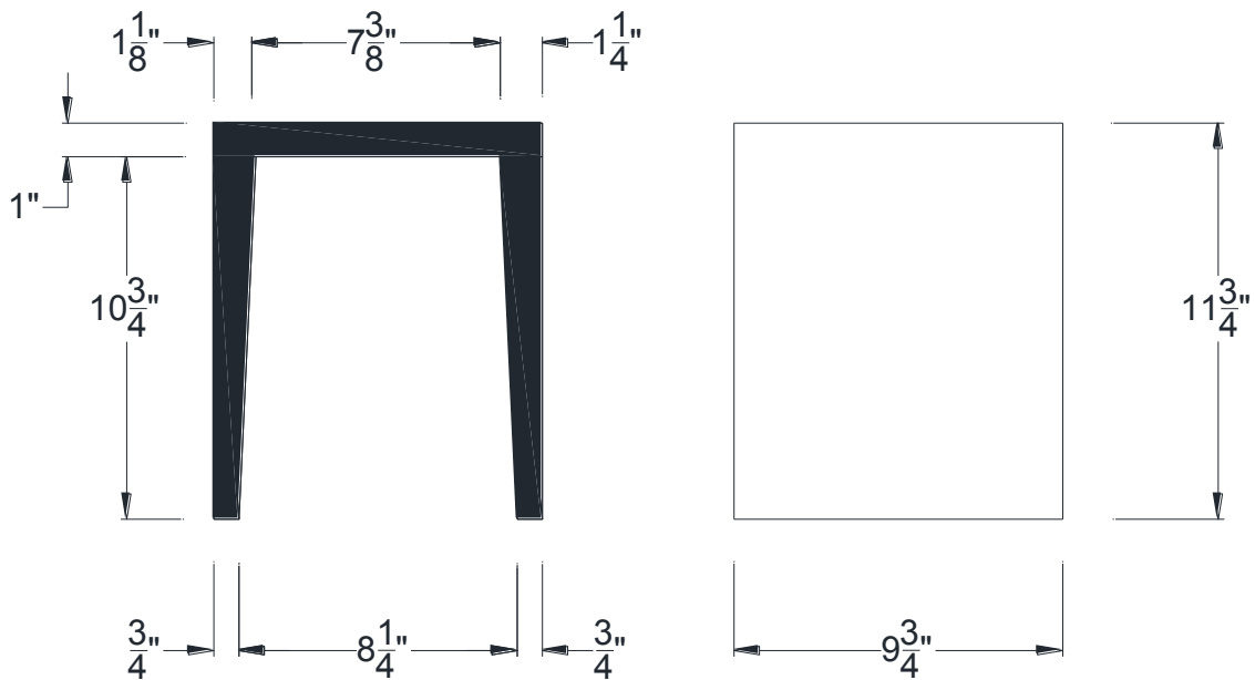
SECTIONAL VIEW
