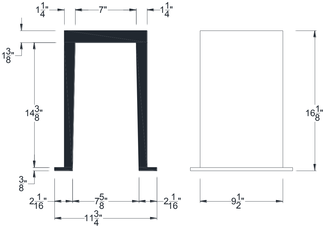
SECTIONAL VIEW
