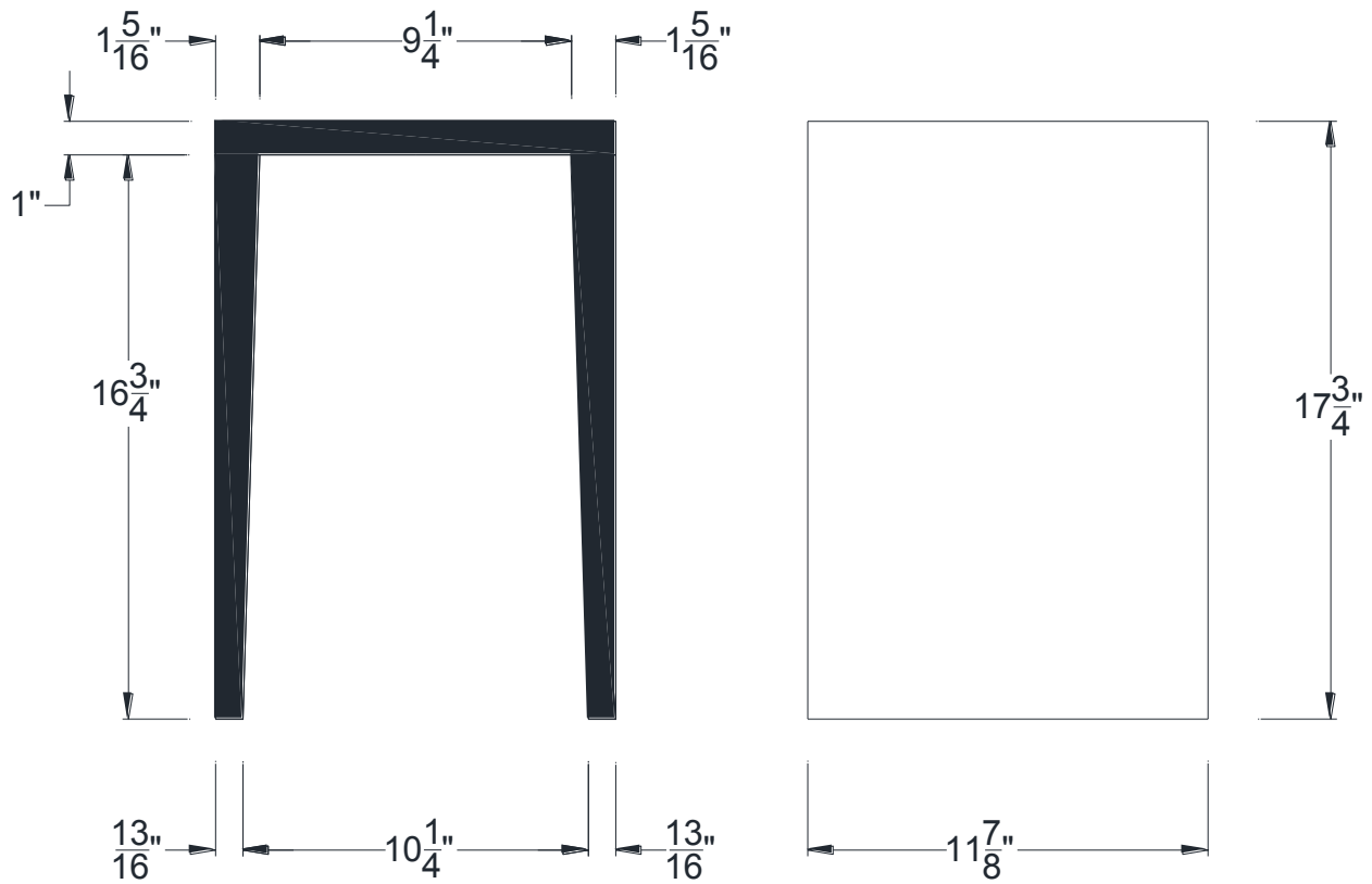
SECTIONAL VIEW
