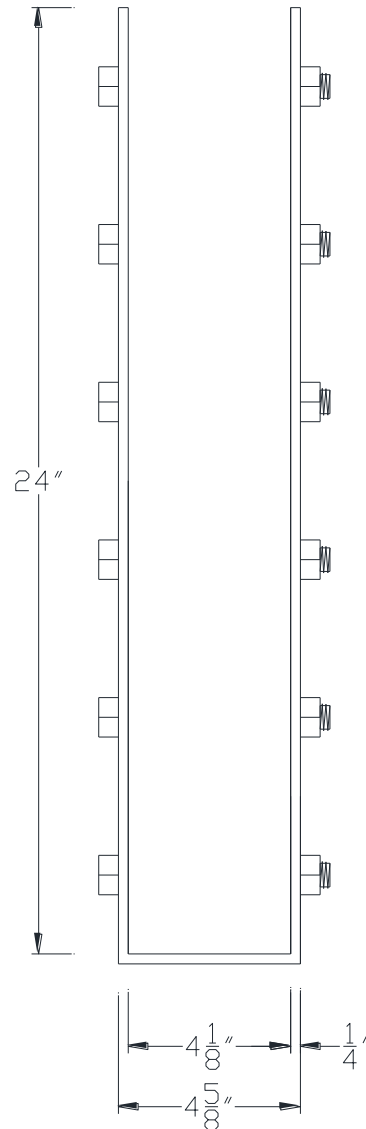
FRONT VIEW
