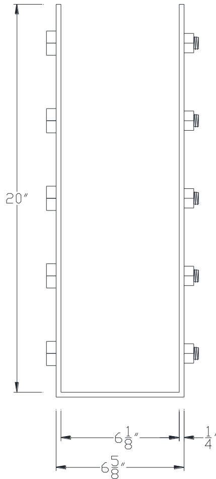
FRONT VIEW
