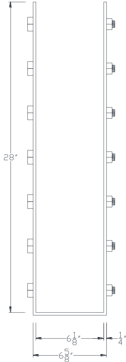
FRONT VIEW
