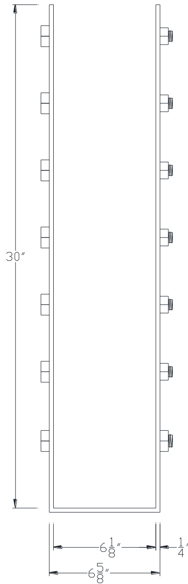
FRONT VIEW
