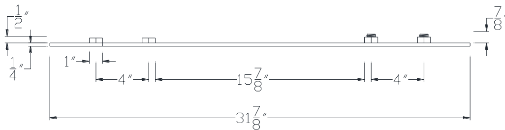
SIDE VIEW
