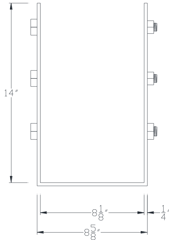
FRONT VIEW
