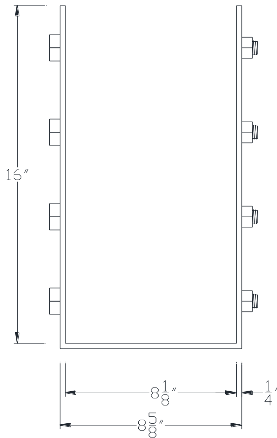
FRONT VIEW
